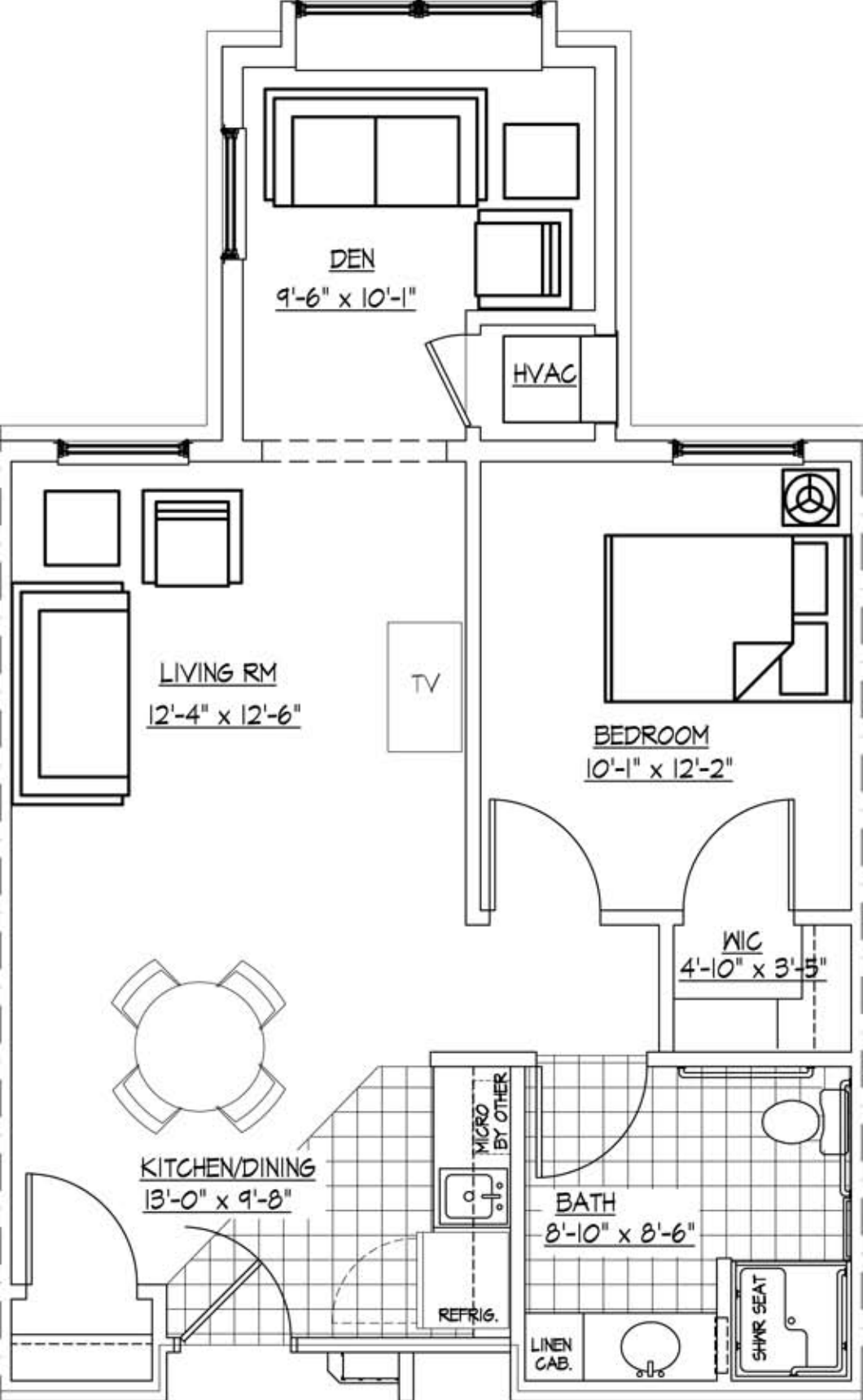
One Bedroom with Den 726 S.F.
